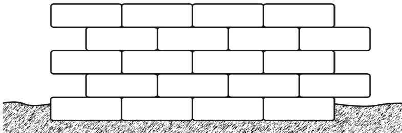
Running Bond Pattern: 3 block per face foot.
