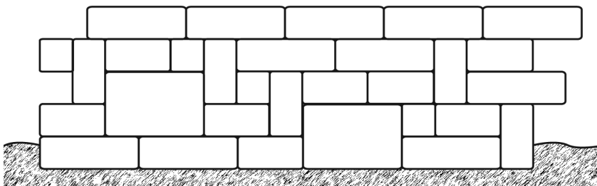
Random Pattern: 3.36 blocks per face foot. Each 20" tall x 60" section uses 28 stones.
